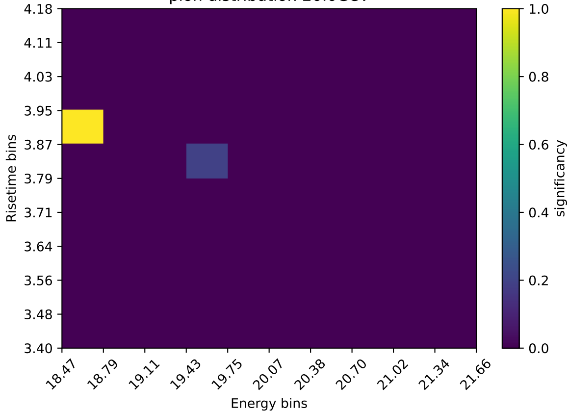
pion distribution 20.0GeV
